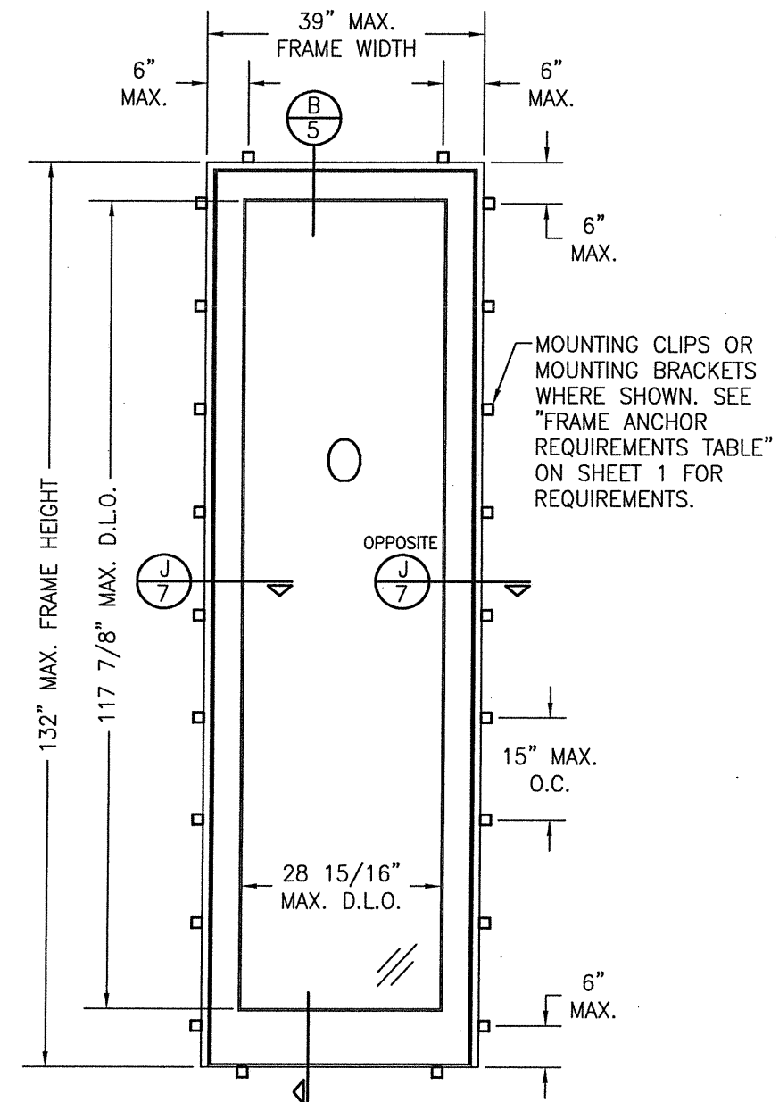
INTERIOR ELEVATION SINGLE FIXED PANEL
