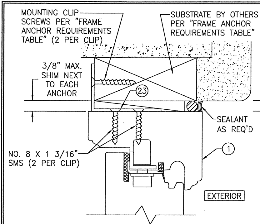
OPTIONAL ANGLE CLIP MOUNT DETAIL AT HEAD
