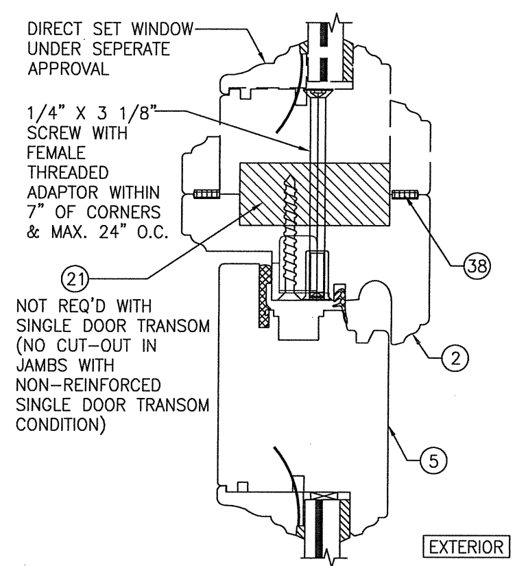
SECTION H2 SCALE: 1/2 FULL (SEE OTHER SECTION FOR DETAIL NOT SHOWN)
