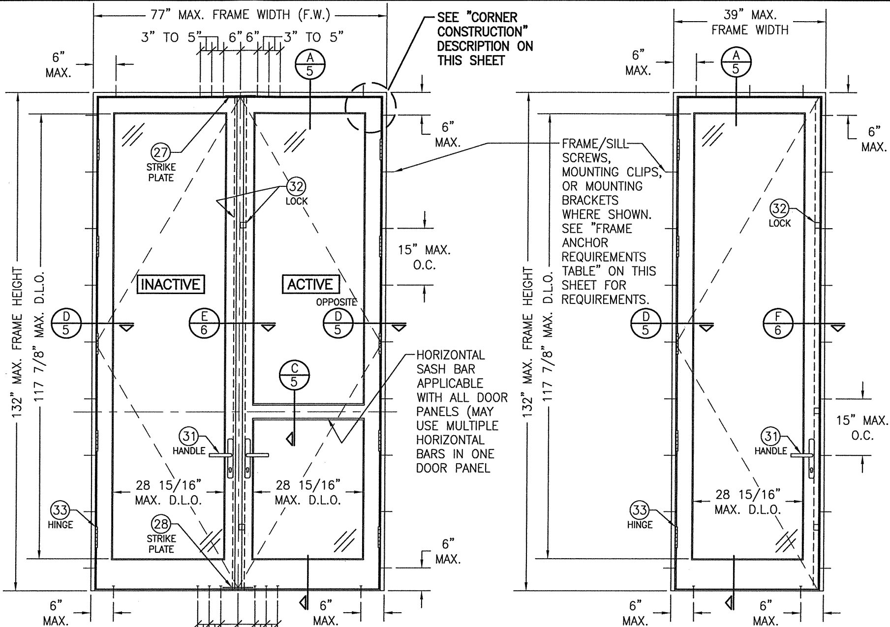
INTERIOR ELEVATION SINGLE RECTANGULAR IN-SWING DOOR
