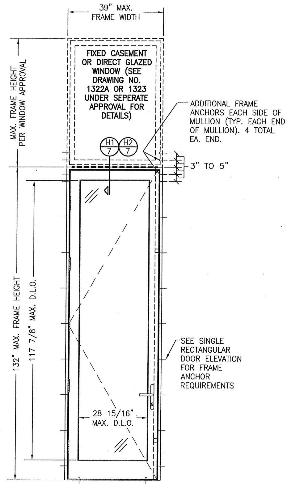
INTERIOR ELEVATION SINGLE DOOR WITH TRANSOM
