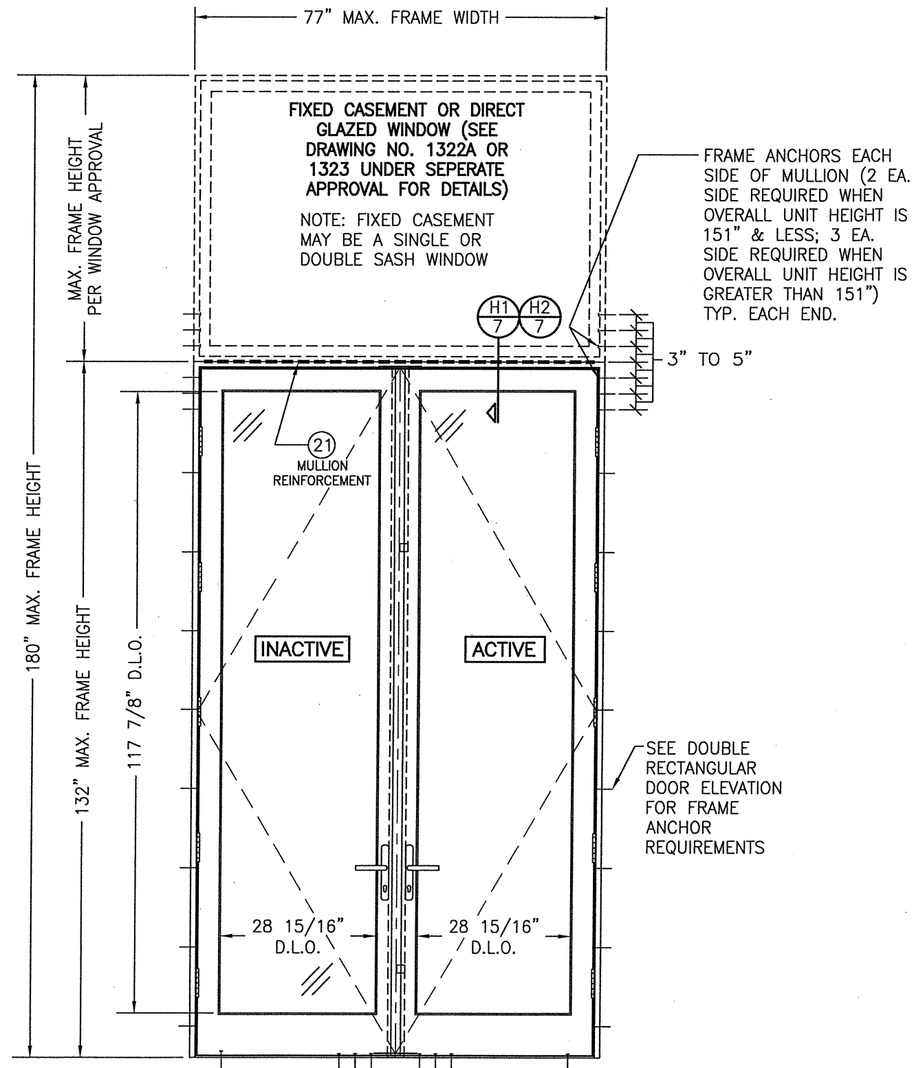
INTERIOR ELEVATION DOUBLE DOOR WITH TRANSOM
