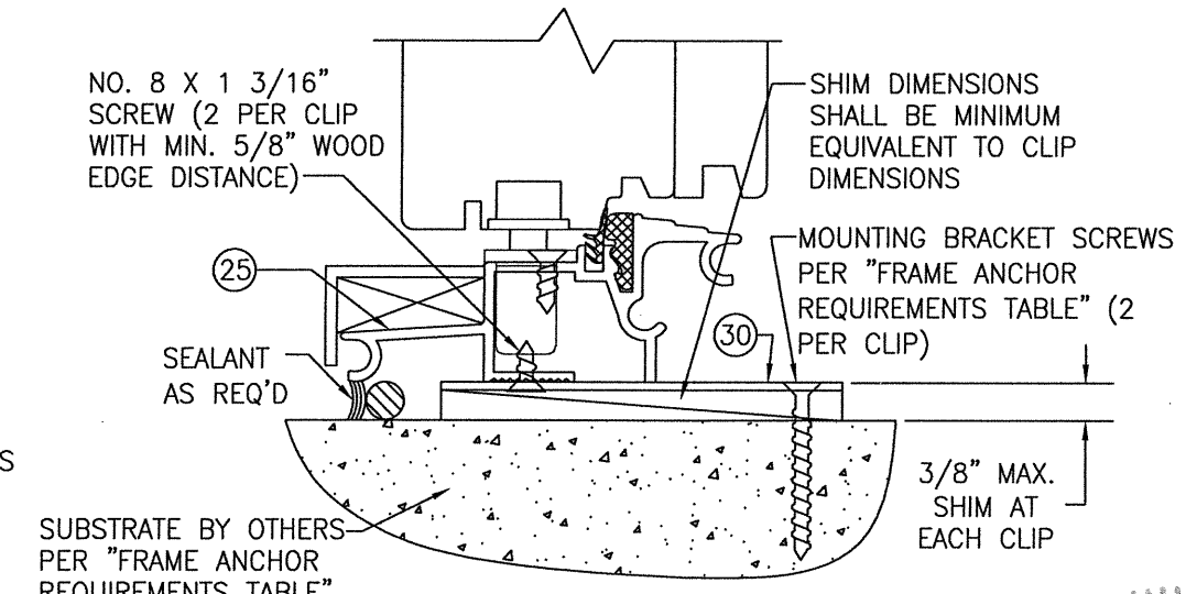
OPTIONAL WIDE INSTALLATION BRACKET MOUNT
