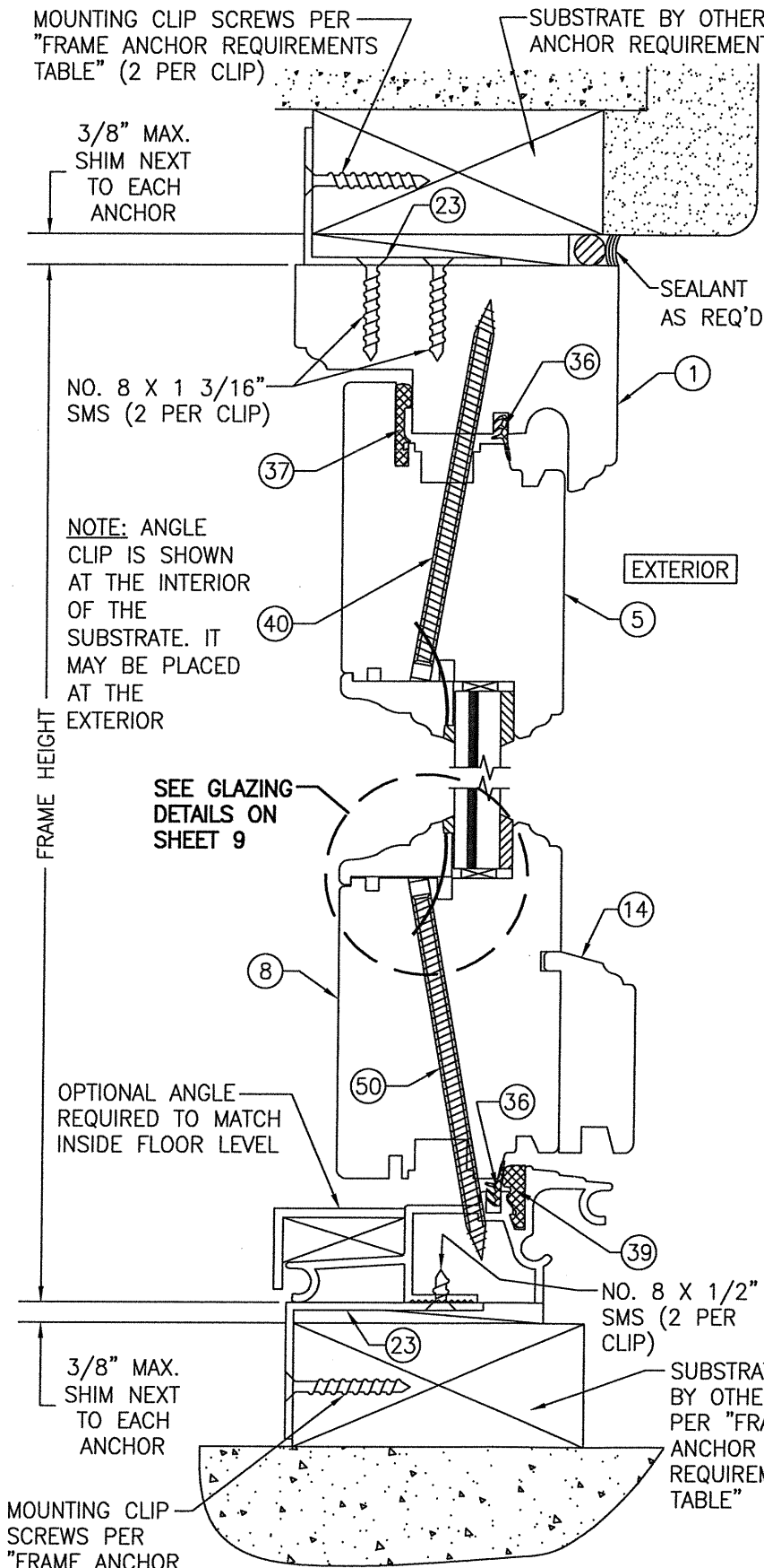
SECTION B SCALE: 1/2 FULL
