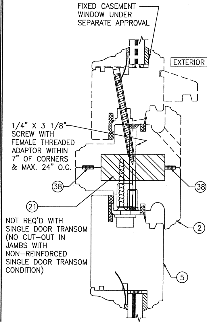
SECTION H1 SCALE: 1/2 FULL (SEE OTHER SECTION FOR DETAIL NOT SHOWN)
