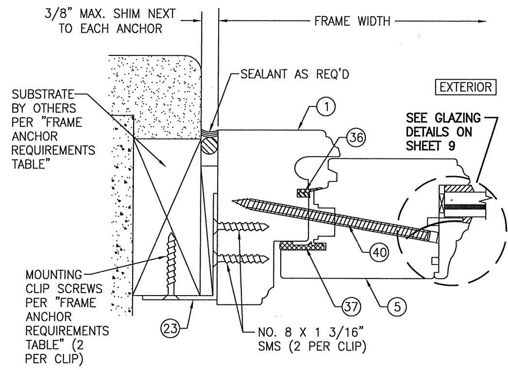
SECTION J SCALE: 1/2 FULL
