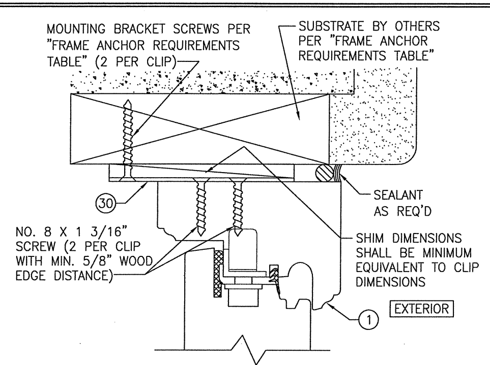
OPTIONAL WIDE BRACKET MOUNT DETAIL AT HEAD
