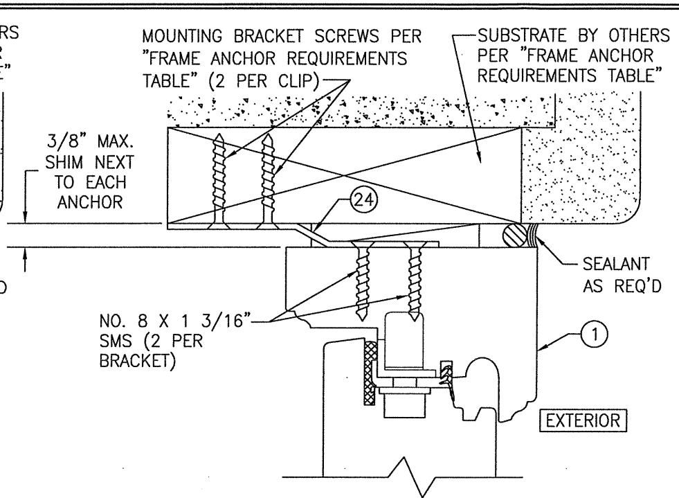
OPTIONAL NARROW INSTALLATION BRACKET MOUNT DETAIL
