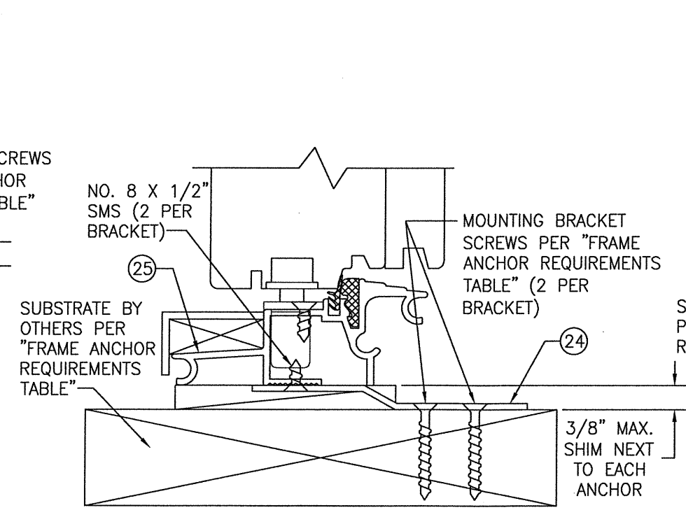
OPTIONAL NARROW INSTALLATION BRACKET MOUNT DETAIL AT SILL
