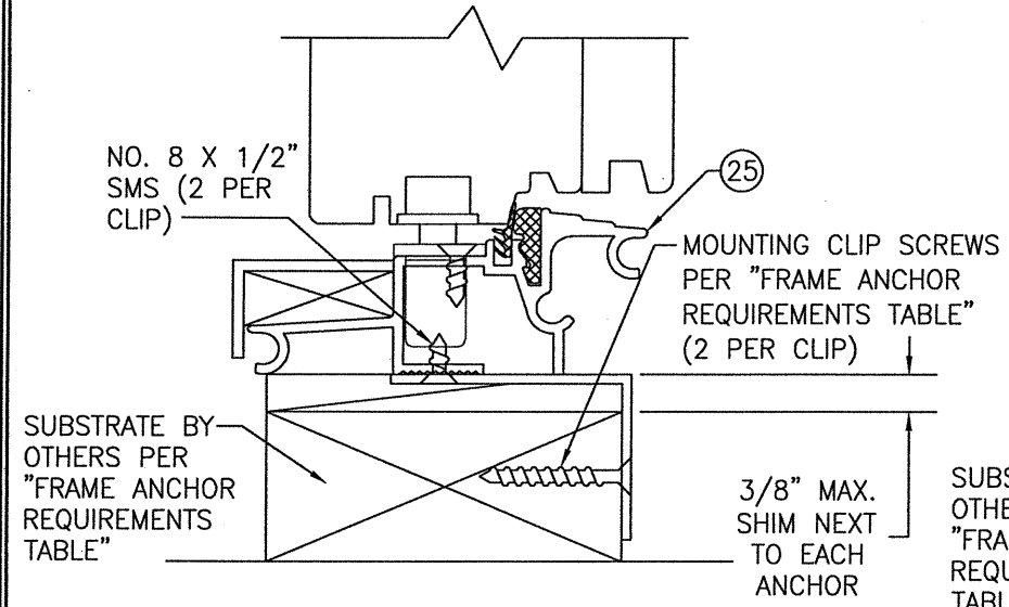
OPTIONAL ANGLE CLIP MOUNT DETAIL AT SILL
